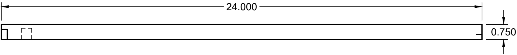
TOP VIEW
